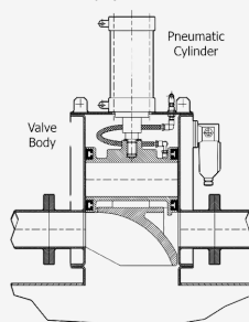
dump position
