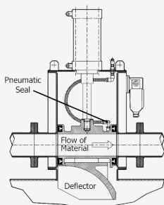
bypass position
