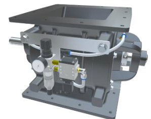
Shaft Air Purge Kit
