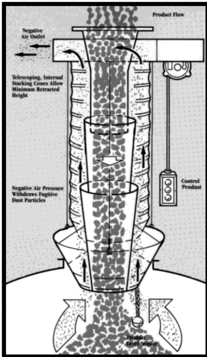
Dry Silo Unloading Spout
